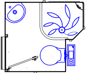
ALISA OPTION B CORNER SINK
